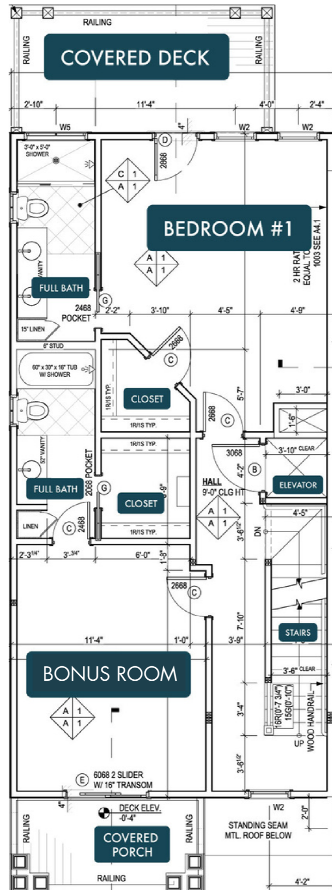
FIRST FLOOR
