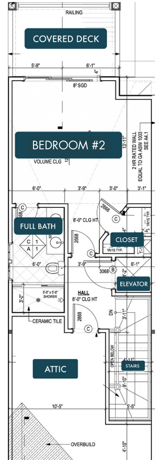
THIRD FLOOR
